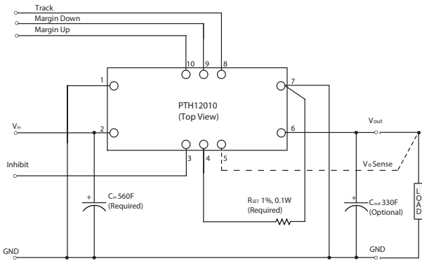
Figure 8 - Standard Application
